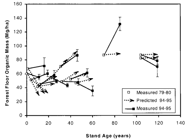
Figure 3. Predicted and observed changes in forest floor organic mass in Federer's chronosequence (1984). These values differ from those reported by Yanai and others (1999, 2000) because a previous error was corrected in the calculation of organic fraction. The starting points differ slightly from Federer's report (see Figure 1) because the archived samples were reanalyzed with the newer samples.
