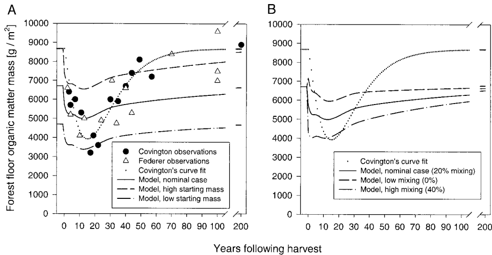
Figure 5. Comparisons of measurements and models of organic mass of the forest floor after harvest. (A) Covington's (1981) and Federer's (1984) measurements shown together with Covington's empirical curve fit, and three simulations of the linked PnET-DocMod models. Model results derive from three different preharvest values of organic mass as steady-state values: our nominal case (6700 g OM/m 2 ), a higher value (8675 g OM/m 2 ) used by Covington (1981), and a lower value (4725 g OM/m 2 ) for illustration. All three simulations used a rate of mixing of 20% of O-horizon organic mass during harvest. (B) Model results from three simulations using our nominal steady-state value of organic mass (6700 g OM/m 2 ), with three different rates of mixing during harvest: 0, 20%, and 40%.
