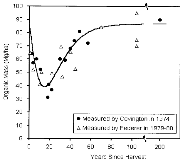
Figure 1. Organic mass of the forest floor in Covington's study (1981) and Federer's additional stands (1984). Covington's curve describes forest floor organic matter (Mg/ha) as -5.25 t^{1.24} \exp(-0.0649 t^{1.063}) + 86.75 , where t = time since logging (years).
