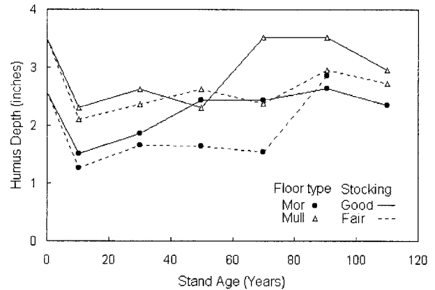
Figure 2. Humus depth as a function of stand age as reported by Sartz and Huttinger (1950). Note that the points for year zero were not observations, but were supposed to describe the humus depth of the former stand prior to logging. The interval up to the first observations was called "a period of organic decomposition following logging."
