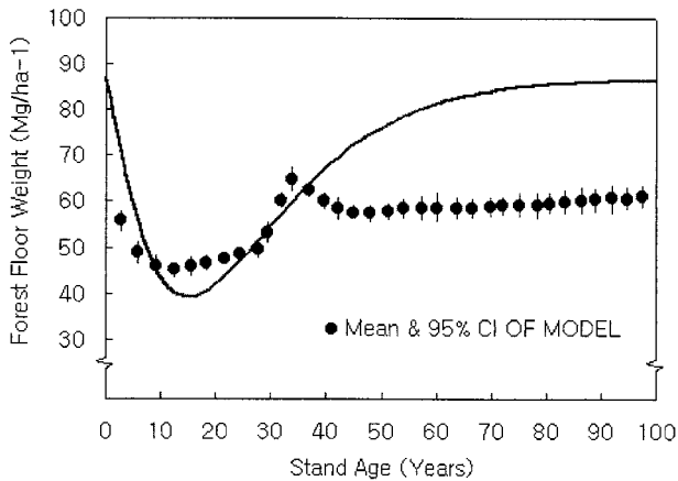
Figure 4. A comparison of the results of the LINKAGES model (Pastor and Post 1986) with Covington's curve (1981).
